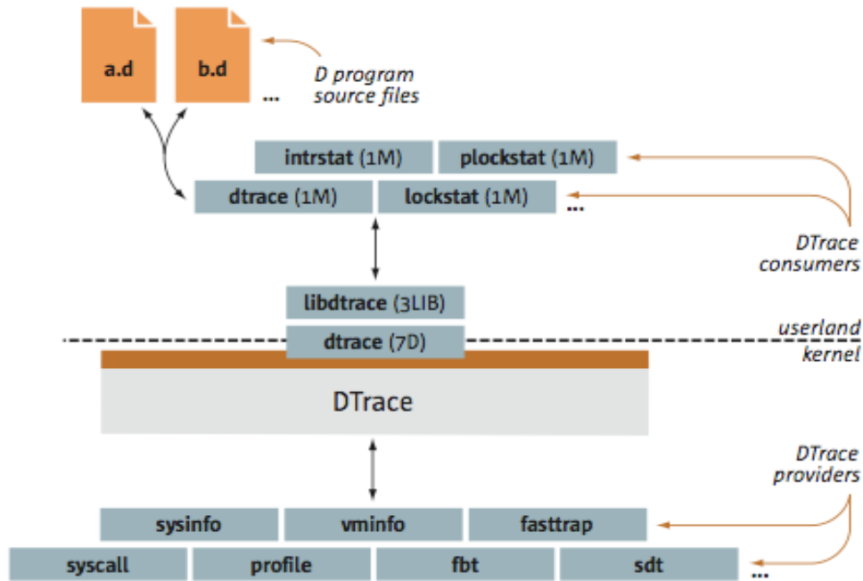
Figure 1—Overview of the Oracle Solaris DTrace Architecture and Components
